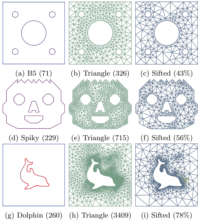
Figure 2: Model, triangle -q35 and sifted meshes.
